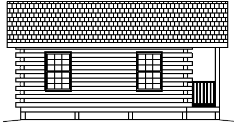
SIDE ELEVATION 1/8" = 1'-0"
