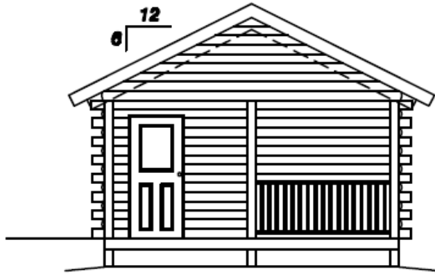
FRONT ELEVATION 1/8" = 1'-0"
