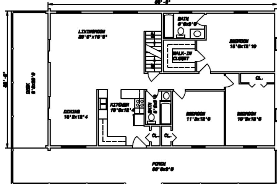
FIRST FLOOR PLAN 1/8" = 1'-0"
