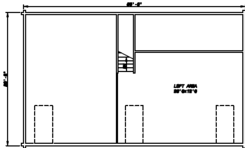
SECOND FLOOR PLAN 1/8" = 1'-0" 28'-6"
