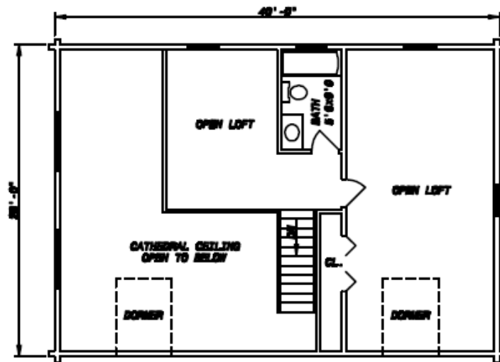
SECOND FLOOR PLAN 1/8" = 1'-0"
