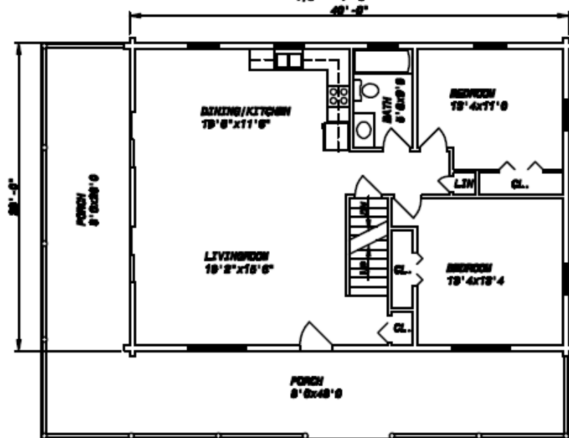
FIRST FLOOR PLAN 1/8" = 1'-0"
