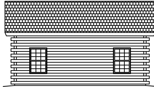
SIDE ELEVATION 1/8" = 1'-0"
