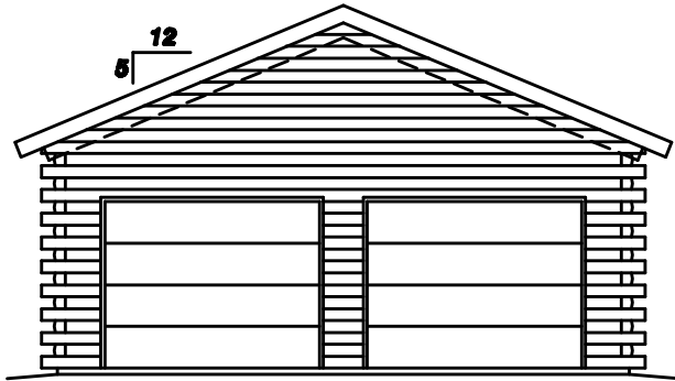
FRONT ELEVATION 1/8" = 1'-0"
