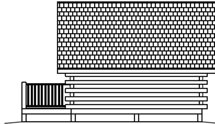
SIDE ELEVATION 1/8" = 1'-0"
