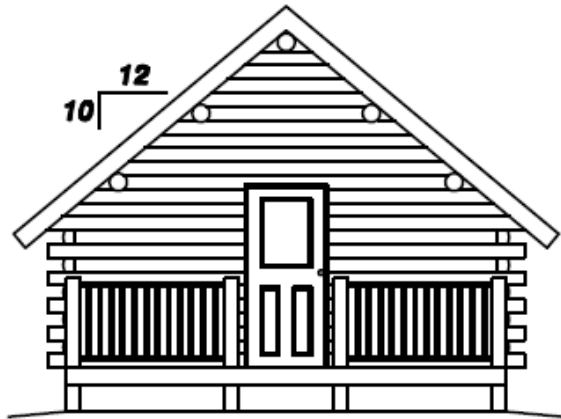
FRONT ELEVATION 1/8" = 1'-0"
