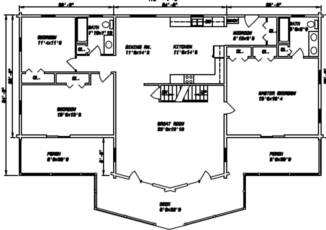
FIRST FLOOR PLAN 1/8" = 1'-0"
